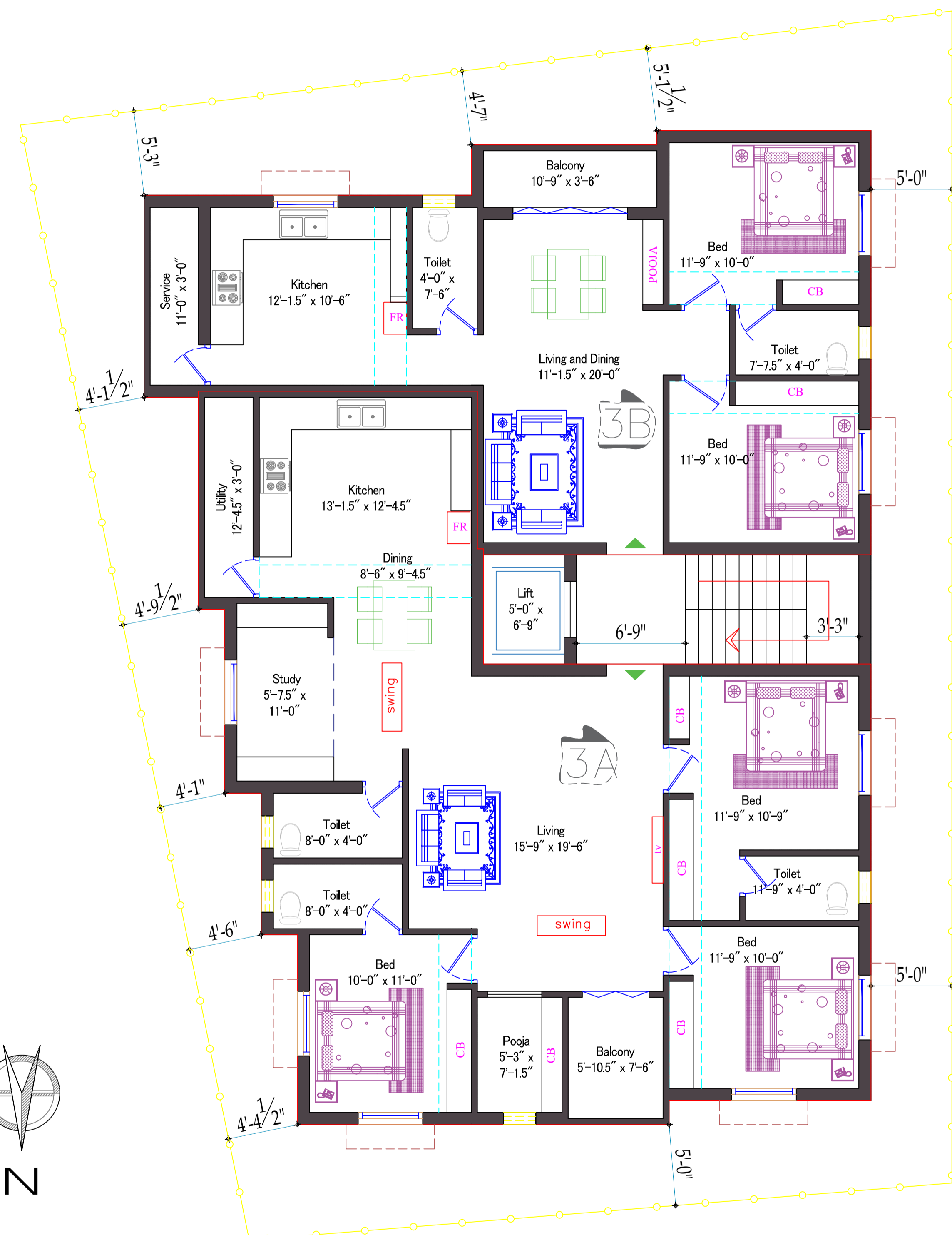
3RD FLOOR PLAN
