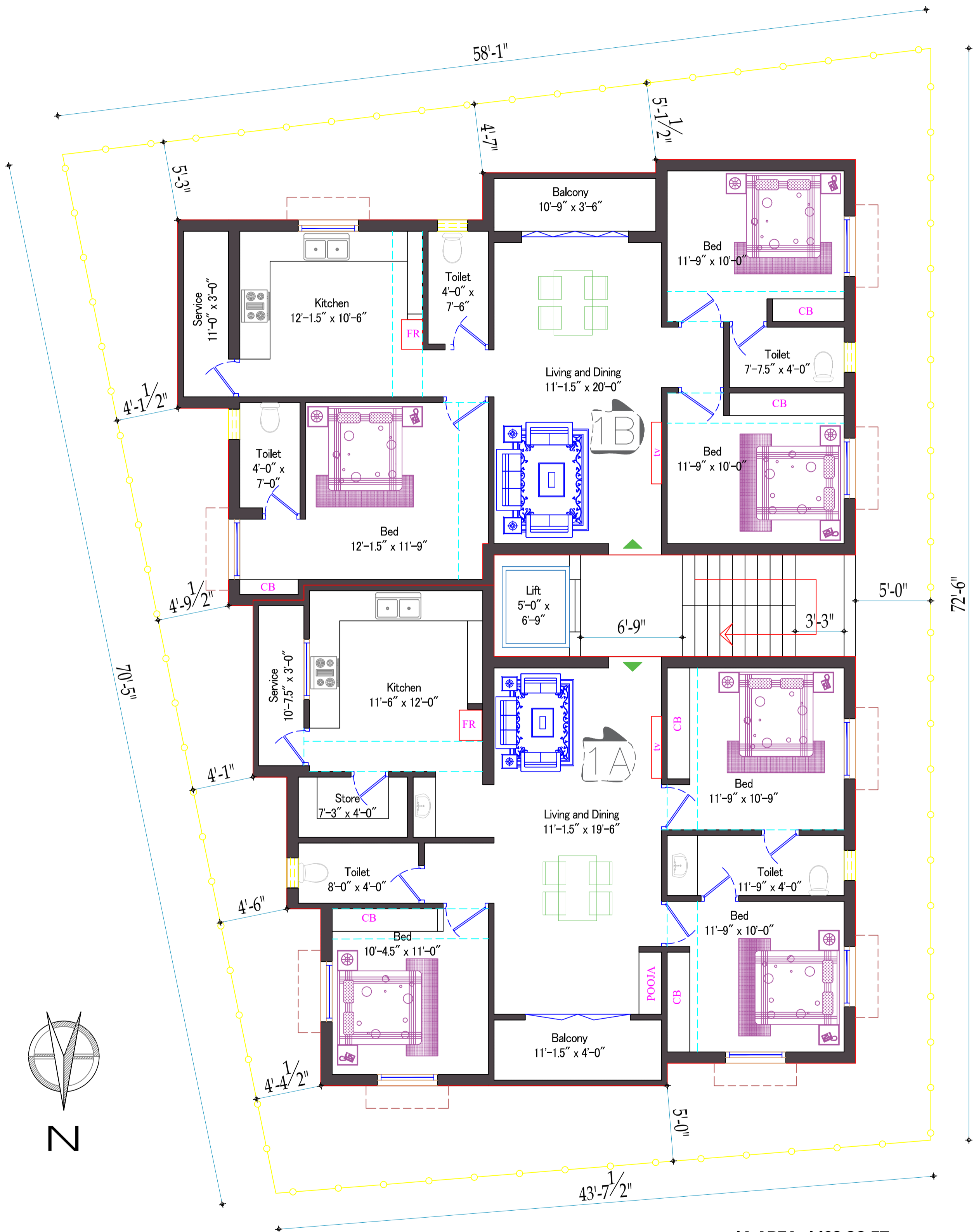
1ST FLOOR PLAN
